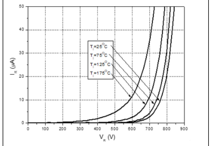
Reverse Characteristics
