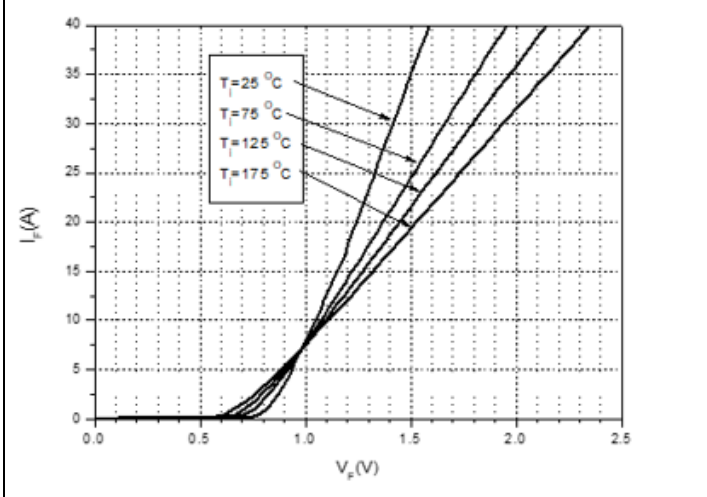
Forward Characteristics
