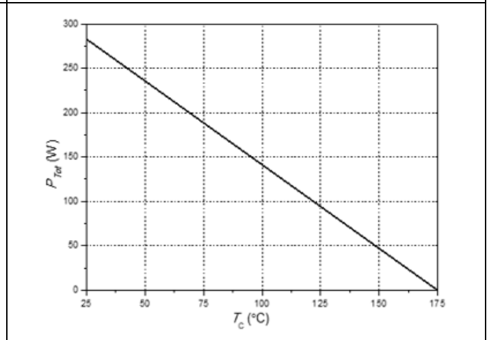
Power Derating
