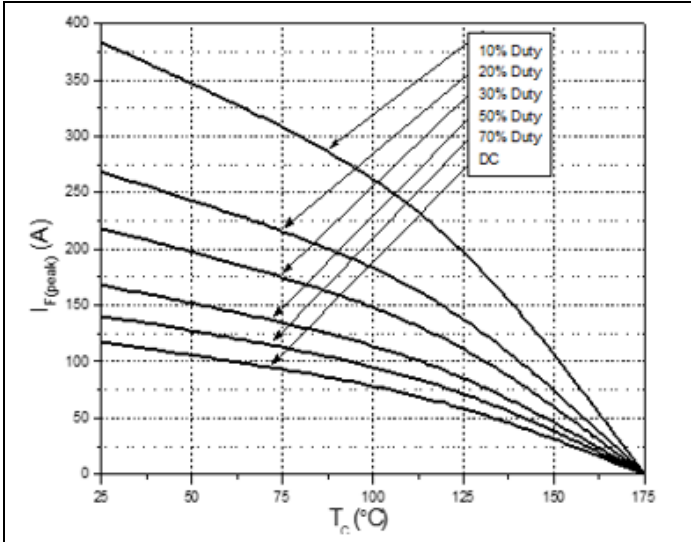
Current Derating
