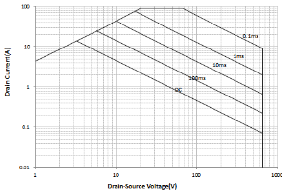
Maximum Safe Operating Area For MS65R135R/TO-247
