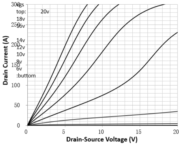
Output Characteristics T_J = -40^\circ\text{C}
