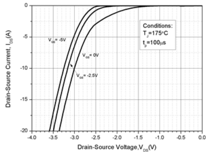
Body Diode Characteristics, T_J = 175^\circ\text{C}
