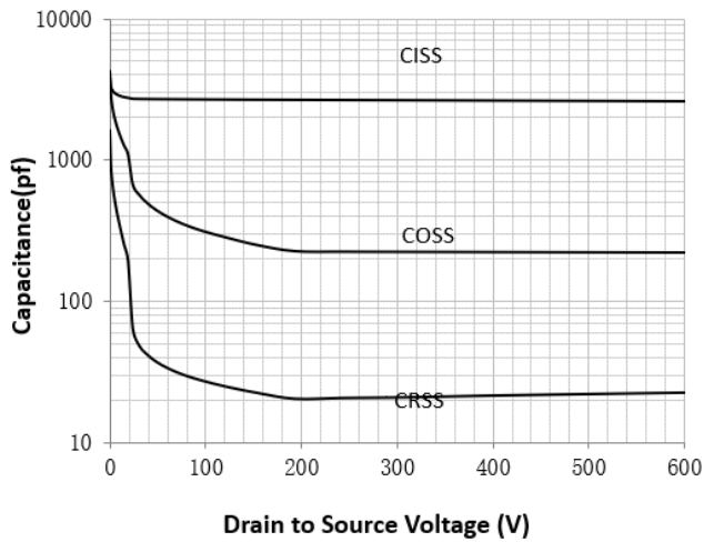
Capacitances vs. Drain-Source Voltage
