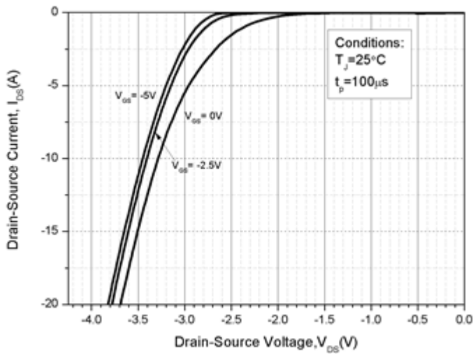
Body Diode Characteristics, T_J = 25^\circ\text{C}
