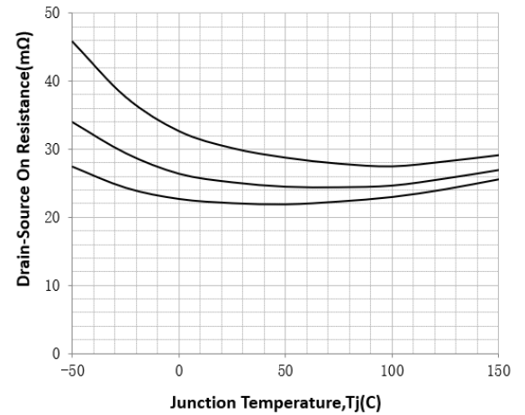
On-Resistance For Various Gate Voltage
