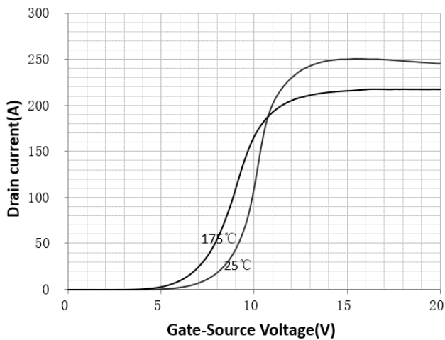
Transfer Characteristic
